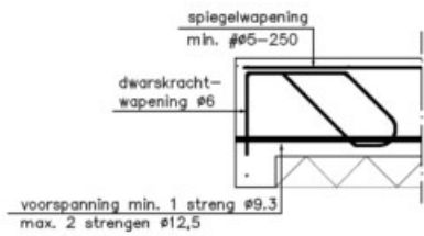
dwarskrachtwapenings detail
